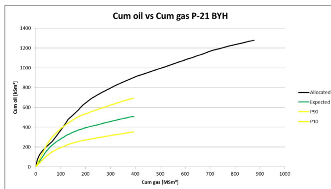
Figure 6: Comparison of modelled and actual cumulative oil production as a function of cumulative gas production
