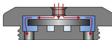
Figure 1: AICD Flow Path
