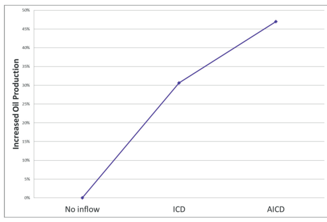
Simulated increase in oil production for ICD and AICD completions
