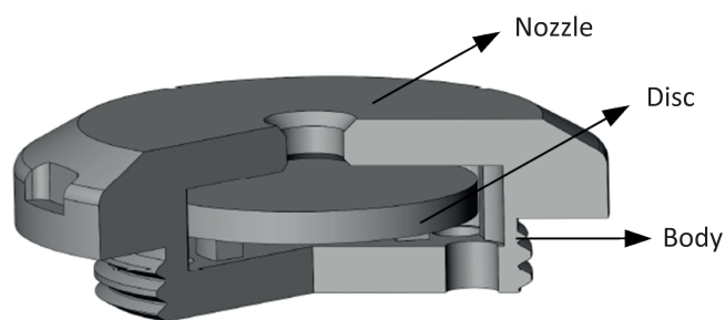
Figure 3: AICD construction
